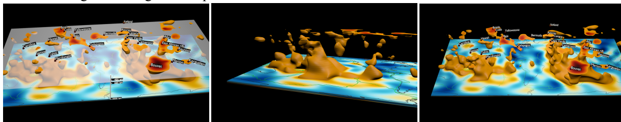
Figure 1.5. Images highlighting the 3-D plume structures, which were shown at the Visualization Showcase at Supercomputing 2016.
