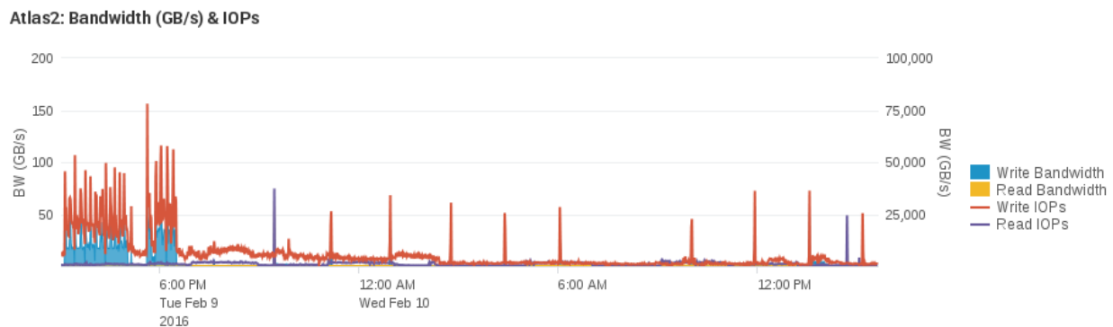
Figure 2.6. Splunk-provided sample of performance data obtained from DDNTool.
